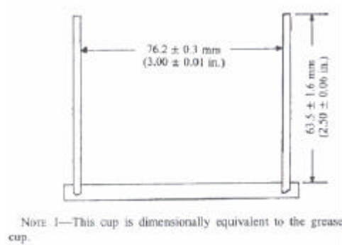
Figure C.1 — Penetrometer cup
