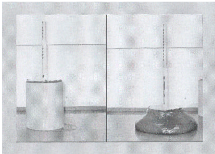
Figure 2 — View of the modified slump test
