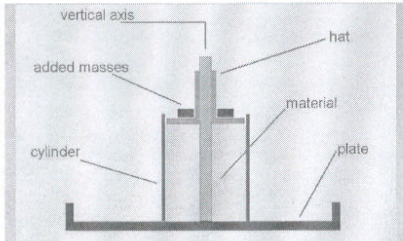
Figure 1 — Detailed scheme of modified slump test
