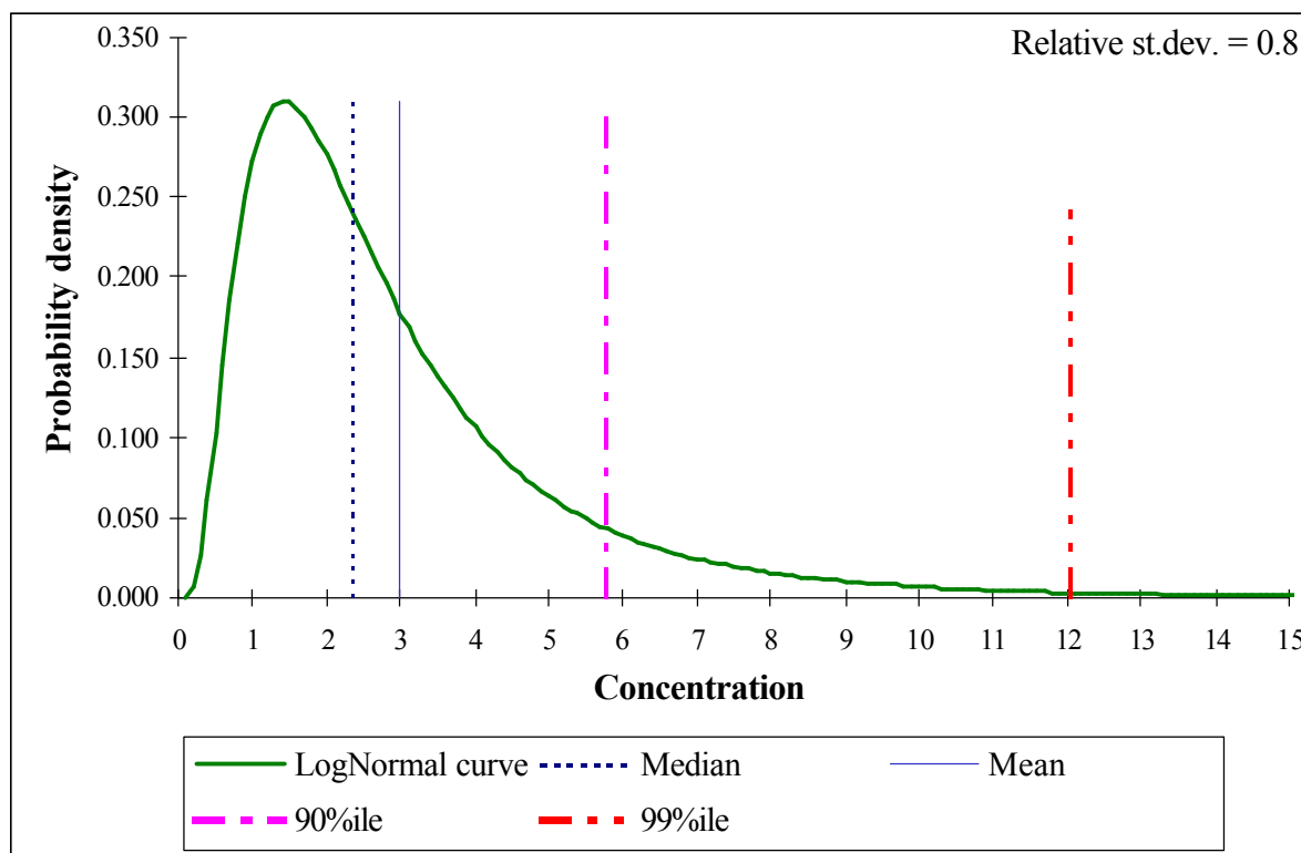
Figure B.2 – Example of a logNormal distribution
