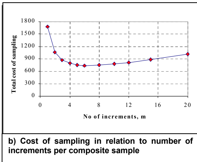
Figure C.1 – Illustration of the relationships between m, n and TC (see text for details)
