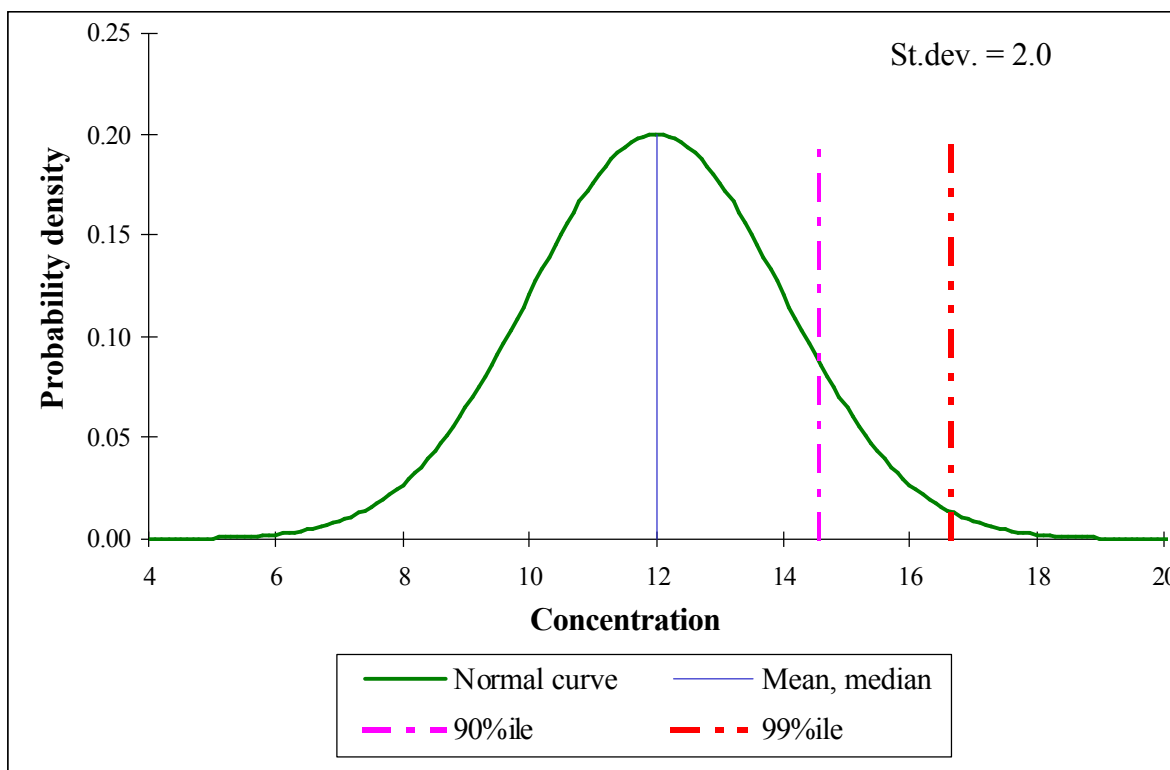
Figure B.1 – Example of a Normal distribution
