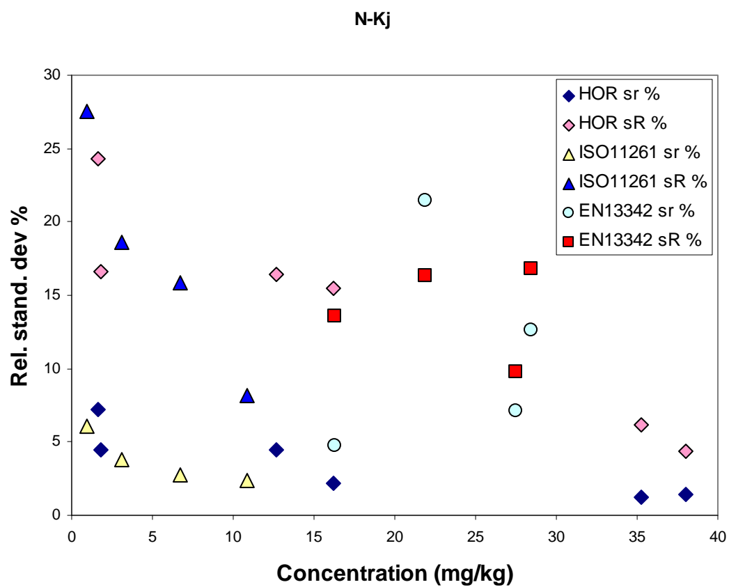
Figure C.1. Within and between lab variability as a function of concentration for NKj. Results from other validation studies using the same method included.
