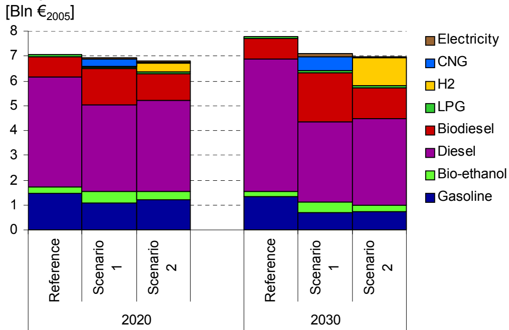
Figure 2 Annual fuel costs road transport
