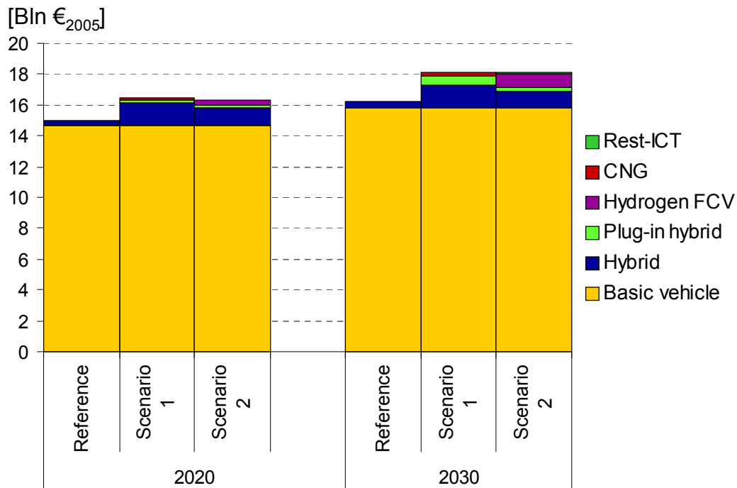
Figure 3 Annual costs vehicle stock 3
